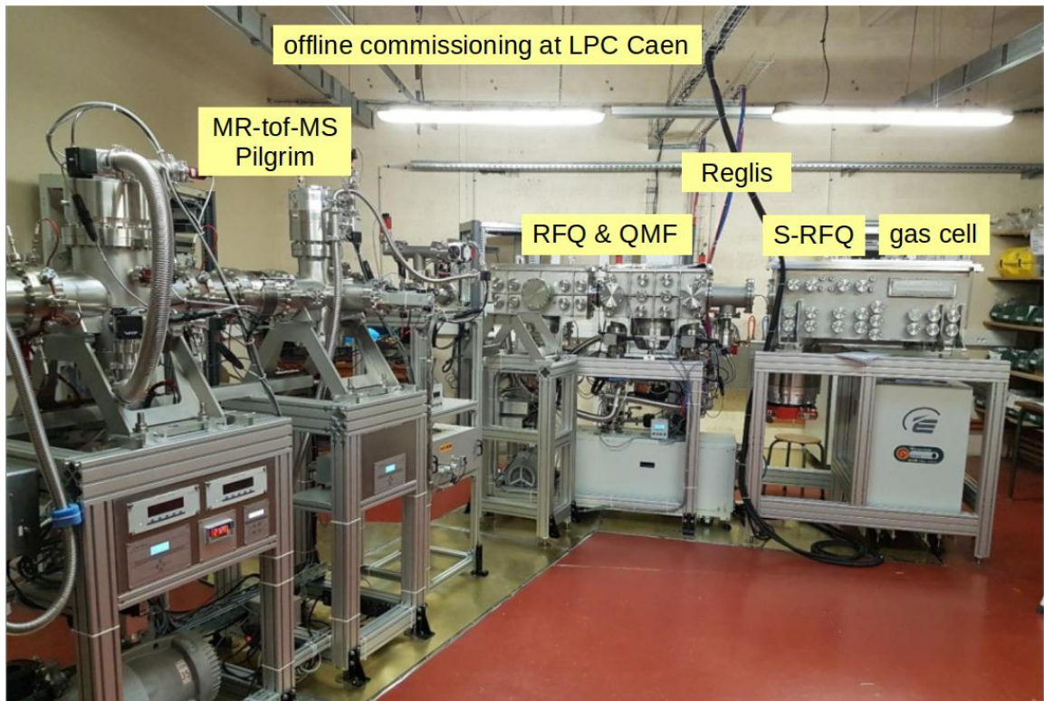
Figure 2. The Reglis and Pilgrim set-ups as they are presently installed at the LPC laboratory in Caen for commissioning
