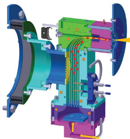
Figure 1. Drawing of the Reglis gas cell. The S3 beam arrives from the left and the gas enters from below (orange). The stopped particles (red) are evacuated on the top right side
