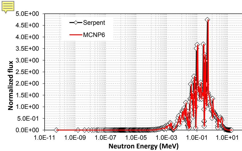
Fig. 2. Comparison of neutron spectra of the CERMET FUELED ADS obtained by Serpent and MCNP6
