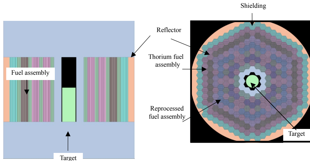
Fig. 1. Vertical and horizontal sectional views of the seed and blanket ADS design
